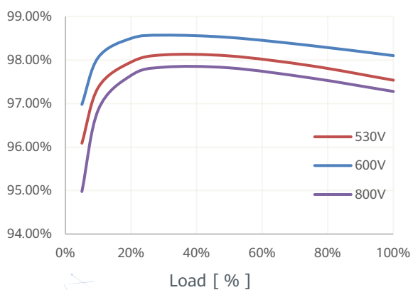
Efficiency Curve
